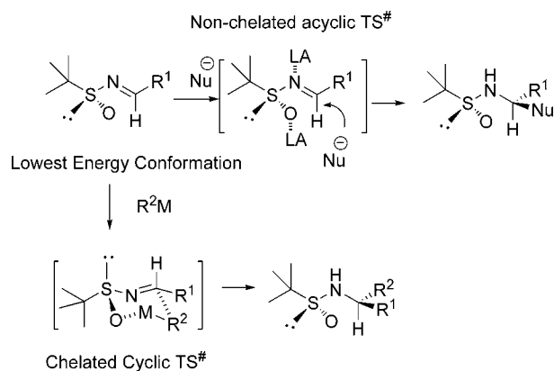
Scheme 1. Mechanistic Models to Predict the Stereochemical Outcomes of the Nucleophilic Additions
