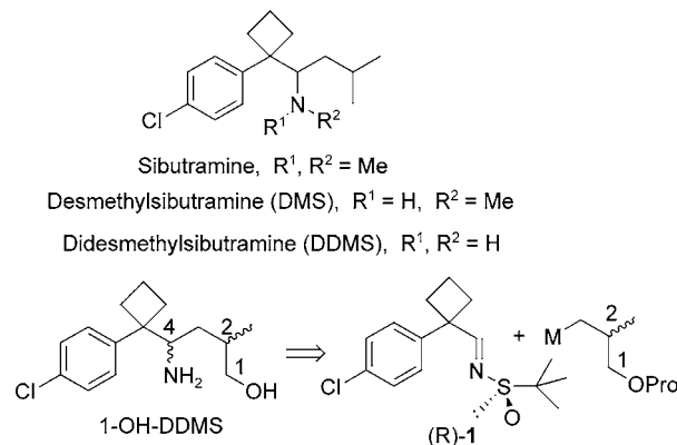
Scheme 2. Retrosynthetic Analysis for Preparation of the Hydroxyl Derivatives of Sibutramine
