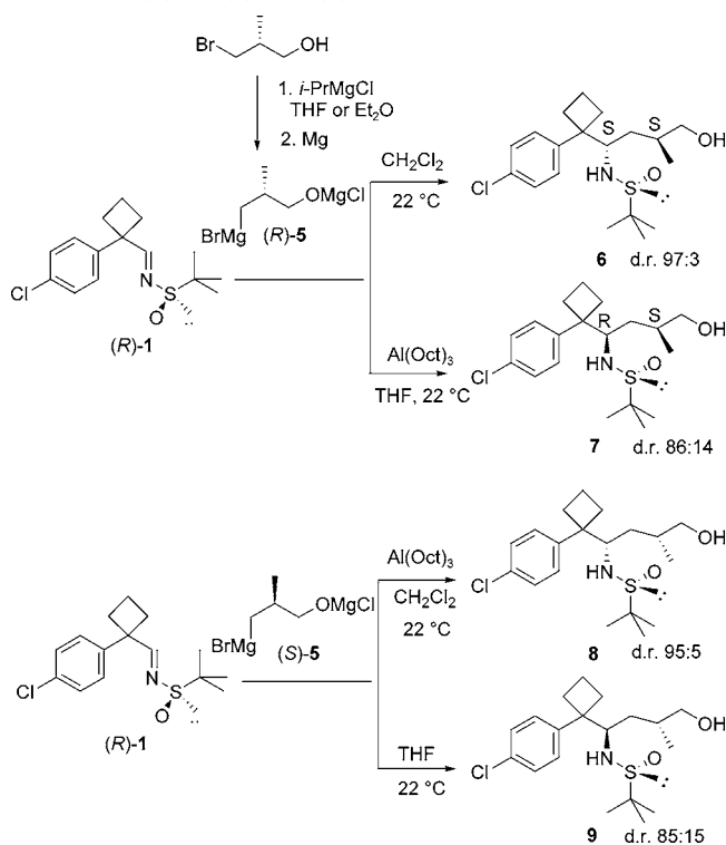
Scheme 4. Diastereoselective Addition of Grignard Reagent ( R )- or ( S )- 5 to ( R )- t -Butanesulfinimine 1
