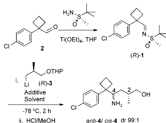
Scheme 3. Diastereoselective Addition of Lithium Reagent ( R )- 3 to ( R )- t -Butanesulfinimide 1
